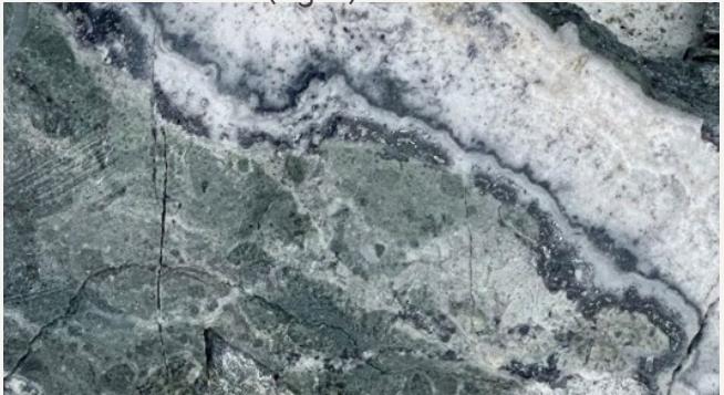
2 Ginguro banding in drill core from CDH-001 (3.00 m @34.7 g/t gold, 3,129 g/t silver from 111 m).
